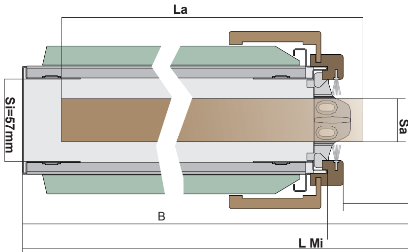
Automatic door operator set
